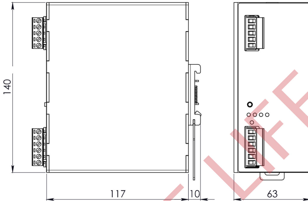
Figure 1. Mechanical Drawing
