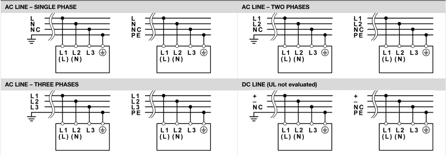
FIG.7 - INPUT CONNECTIONS
